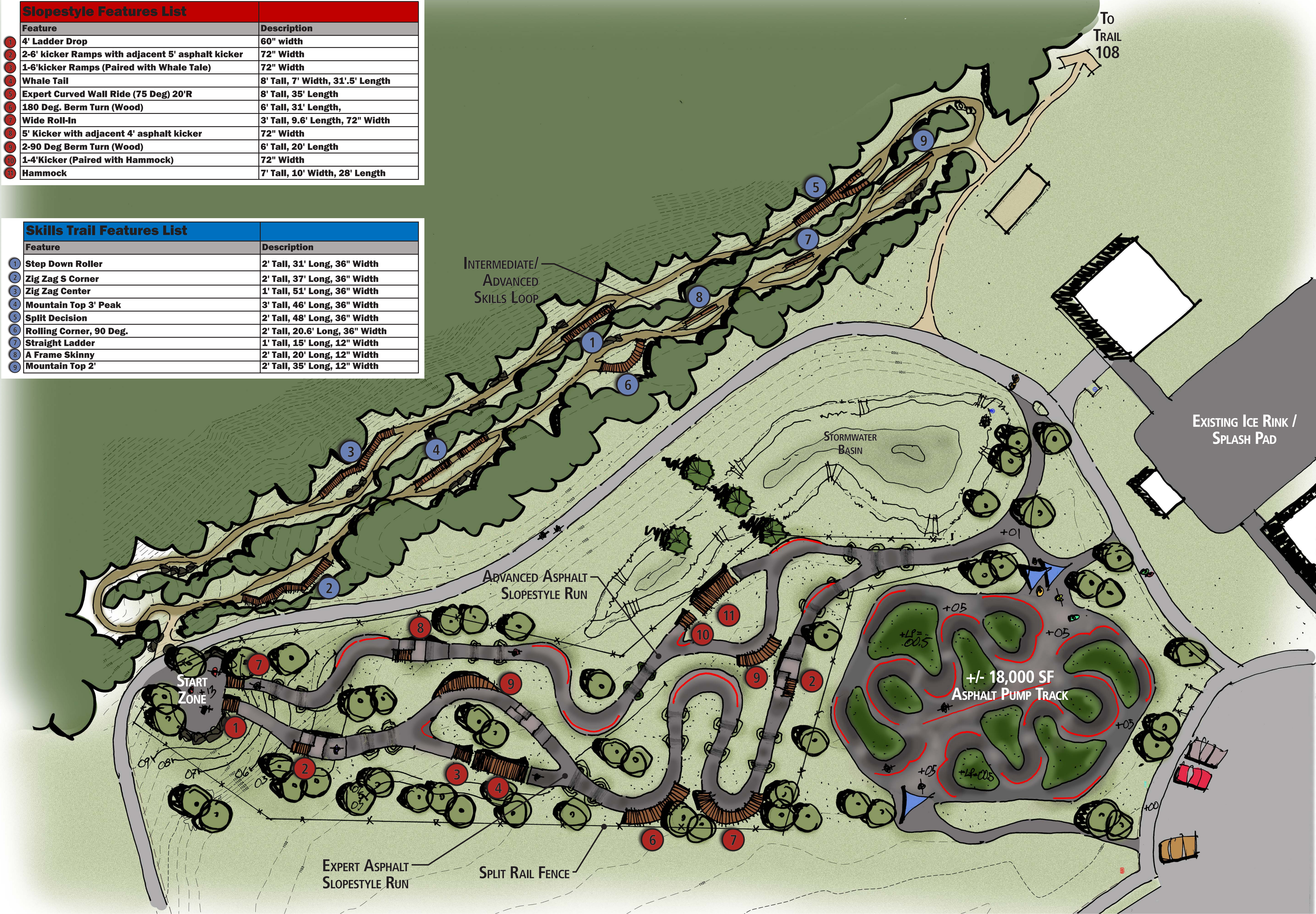
CONE PARK - BIKE PARK PUMP TRACK, SLOPESTYLE LINES AND INTERMEDIATE SKILLS LOOP - SCHEMATIC DESIGN
